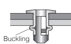
Cross-sectional diagram of riveted boards
